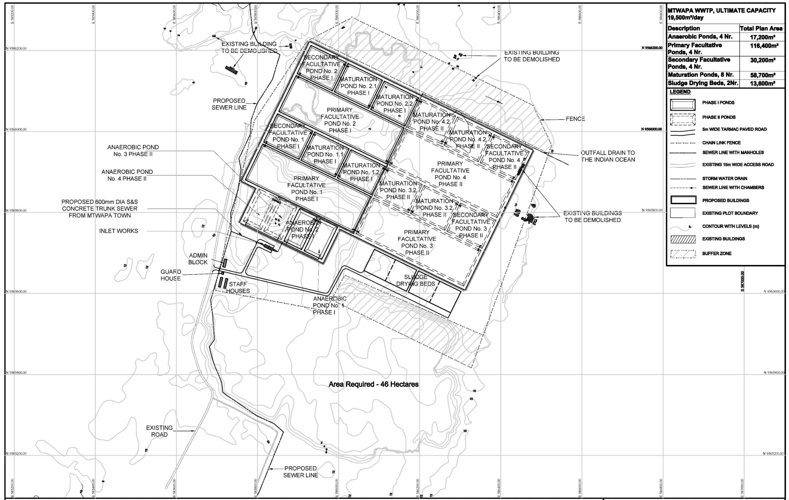
Figure 10.5: Site Layout Plan of the Proposed Wastewater Treatment Plant
