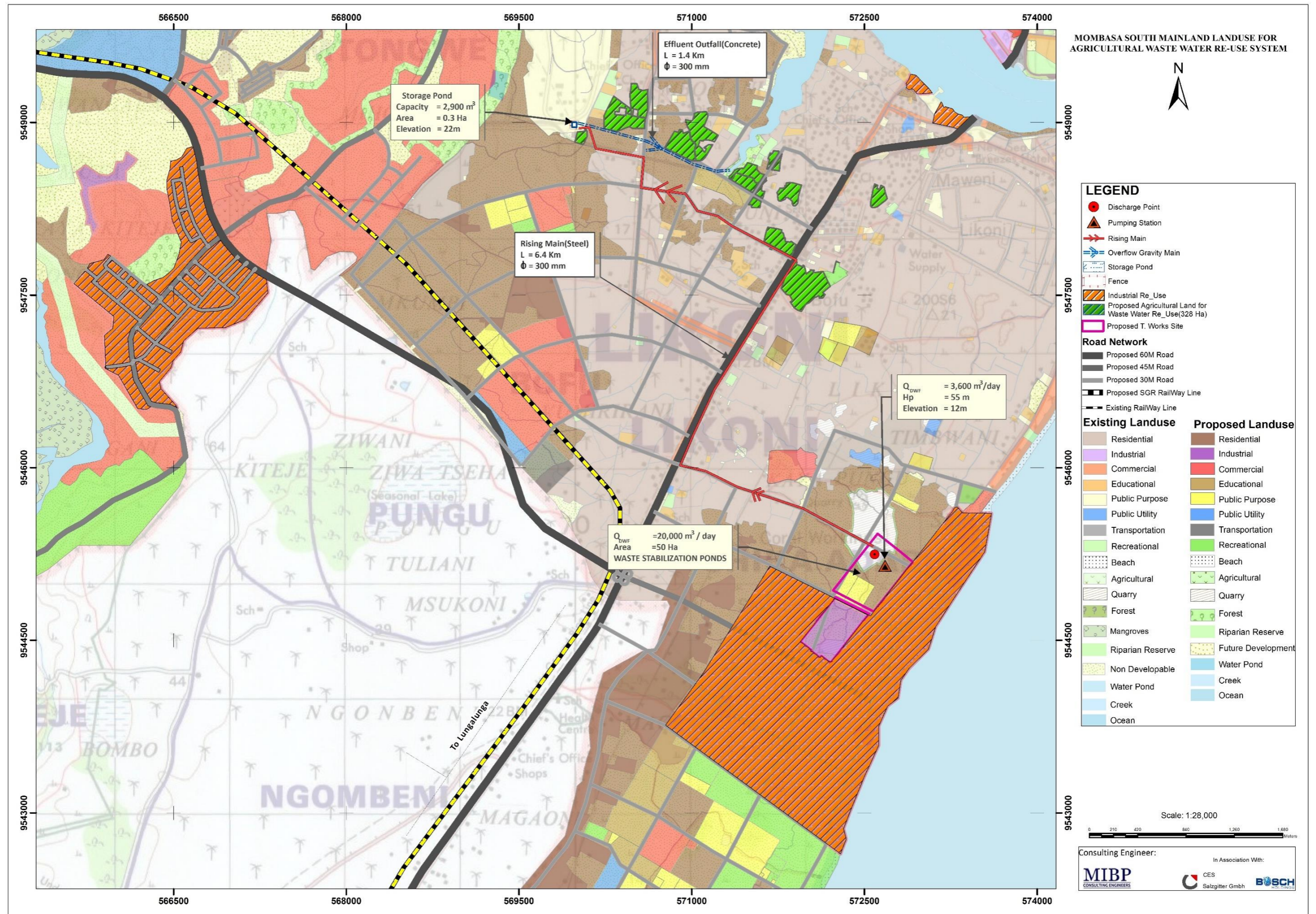
Figure 10.9: Layout Plan of the Conveyance and Storage System for Agricultural Wastewater Reuse – Mombasa South Mainland
