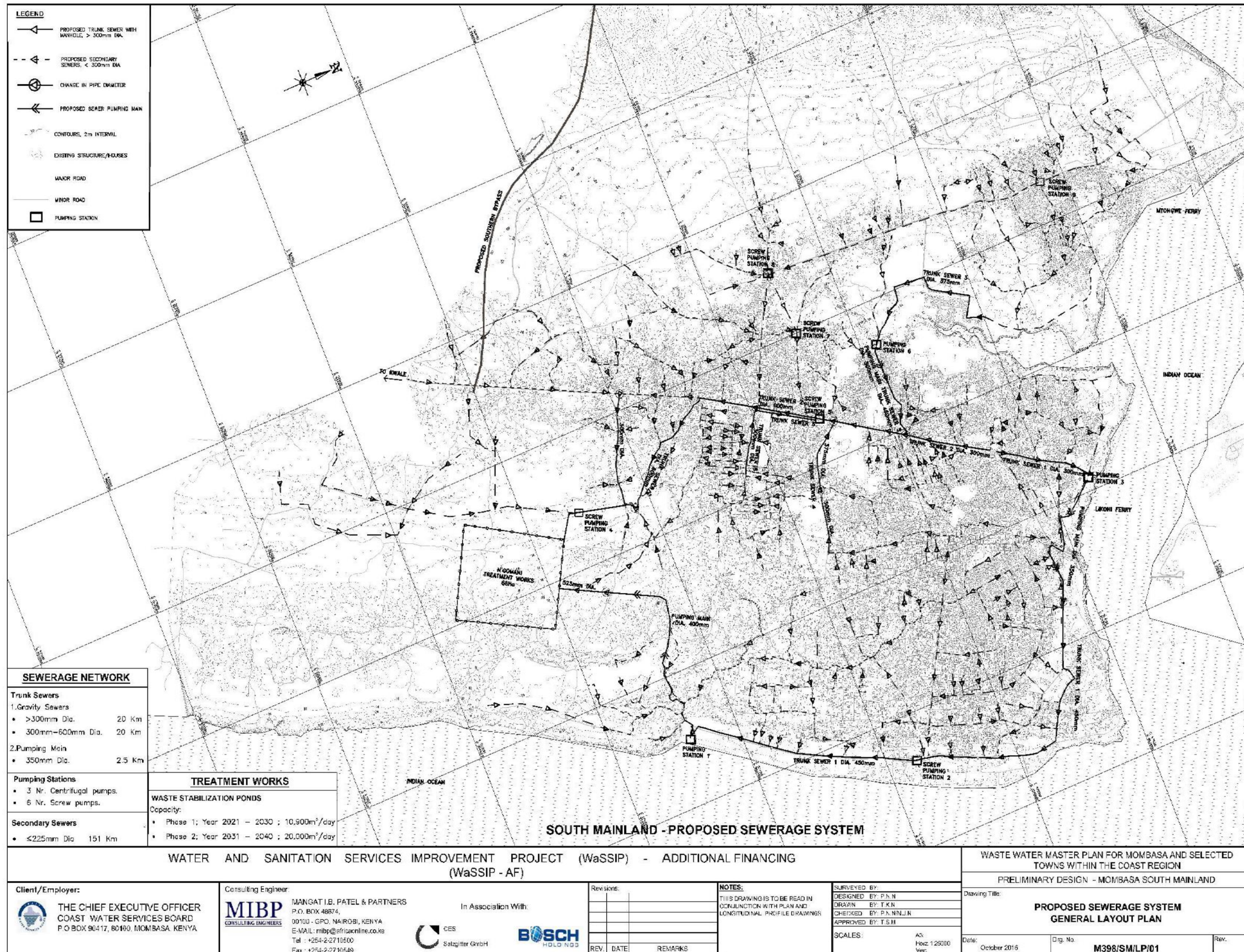
Figure 10.1: Detailed Layout of the Sewerage System
