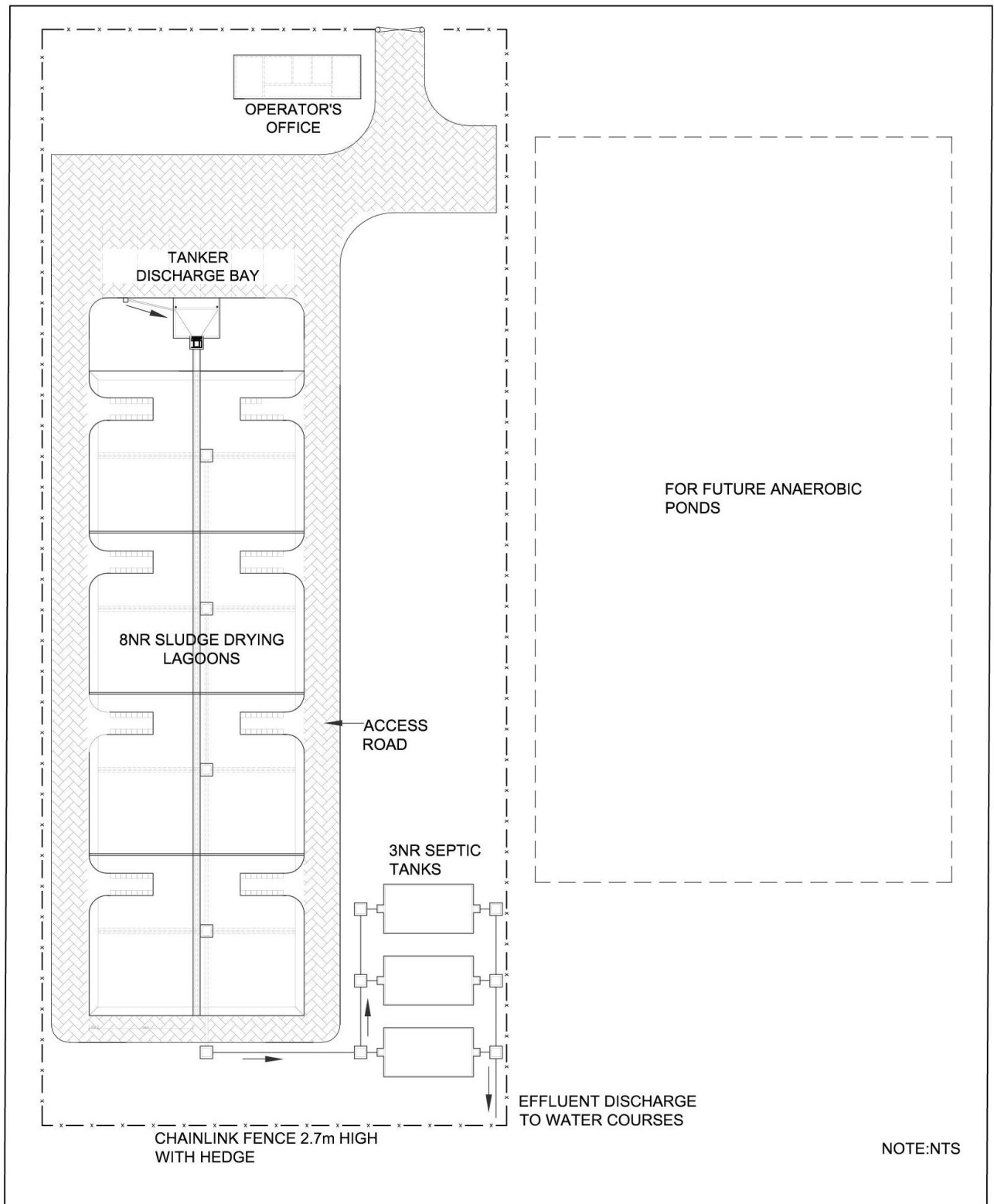
Figure 2.5: Schematic Layout Plan of the proposed Sludge Handling Facility
