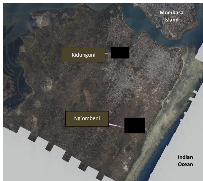
Figure 7.5: Locations of Candidate Sites for Wastewater Treatment Plant Sites
