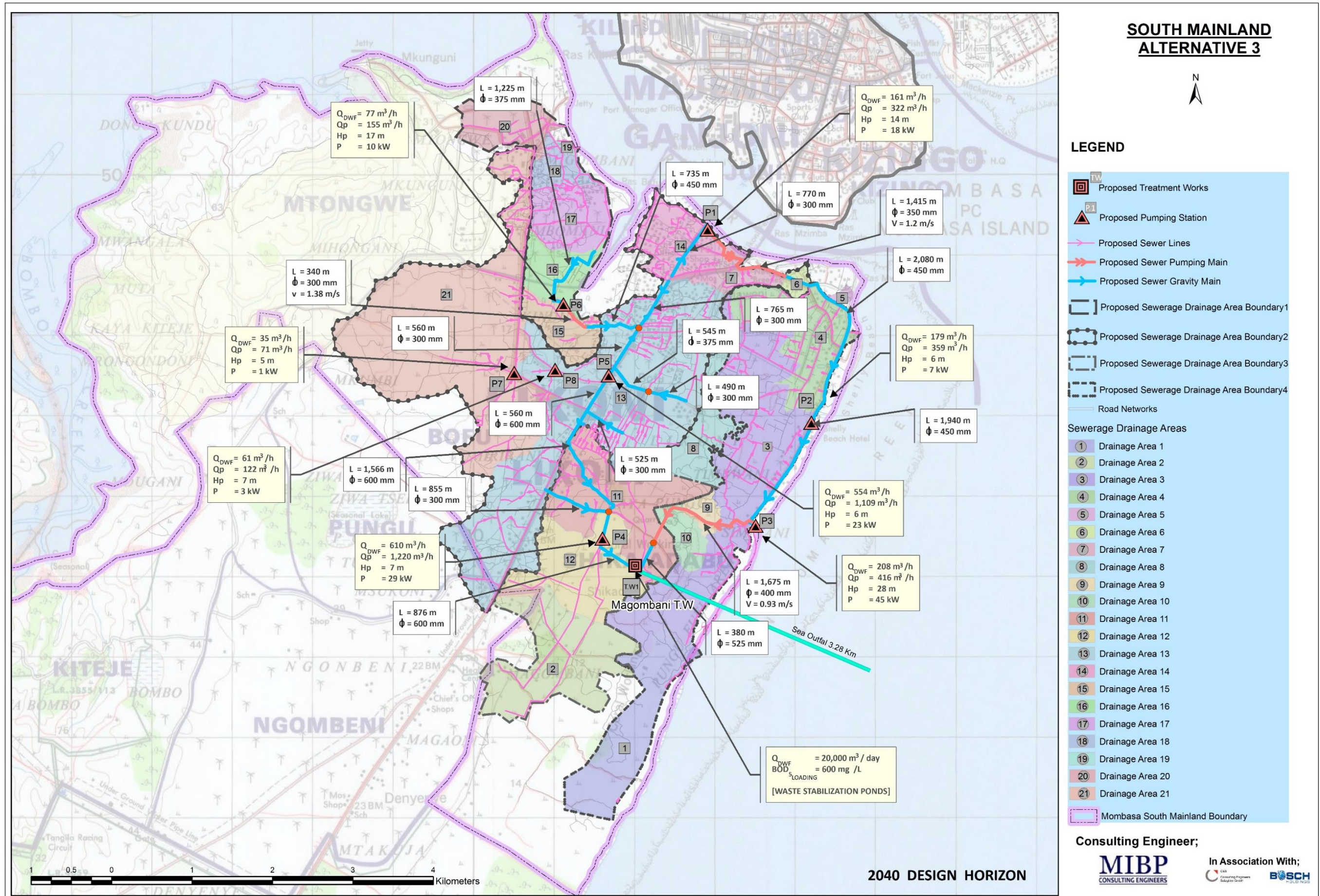
Figure 7.4: Alternative Scheme 3
