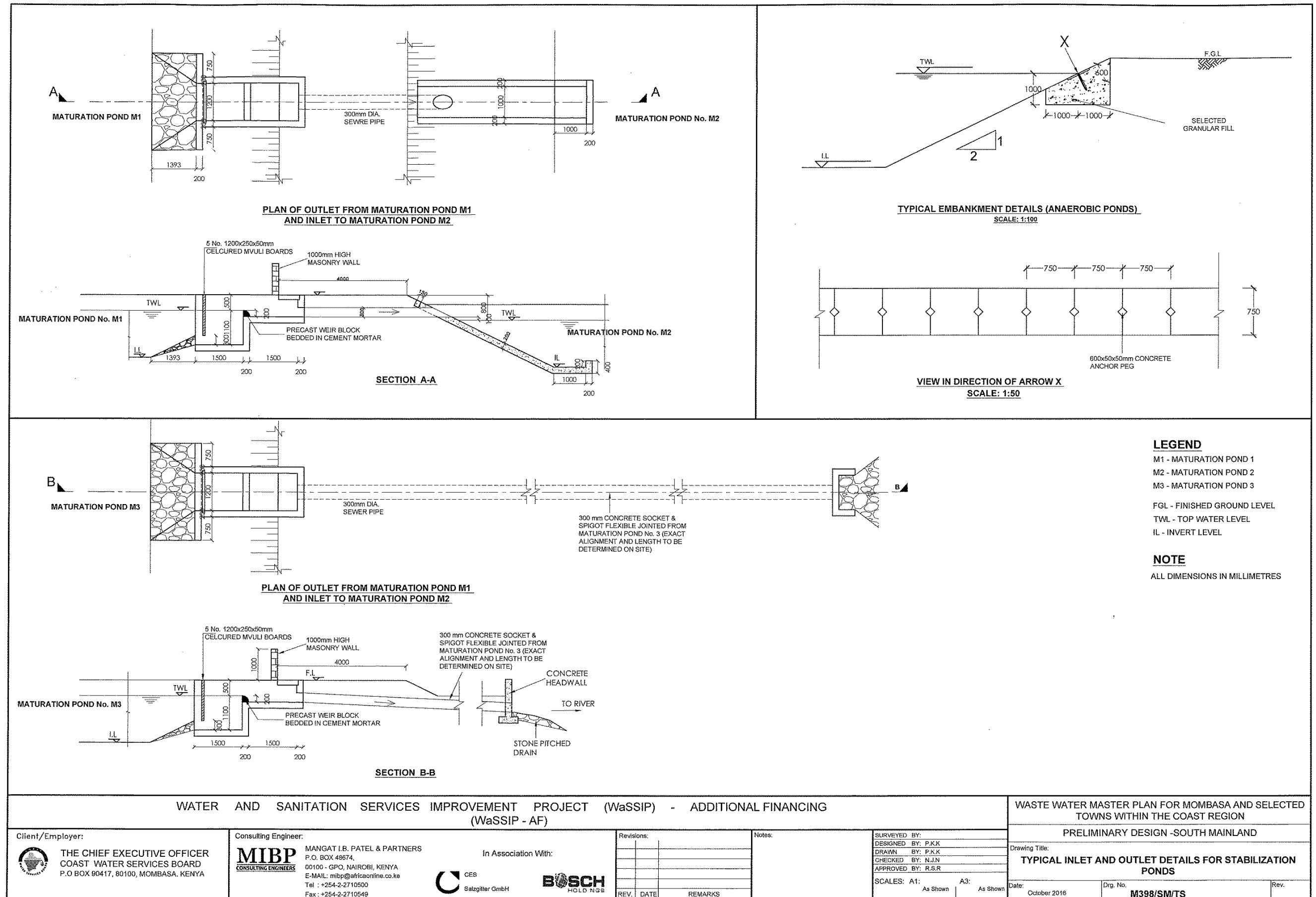
Figure 10.6: Typical Inlet and Outlet Structures for the Ponds
