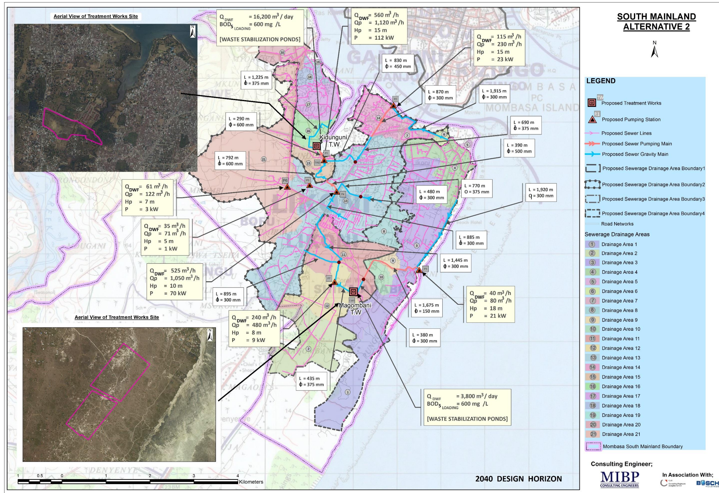
Figure 7.3: Alternative Scheme 2
