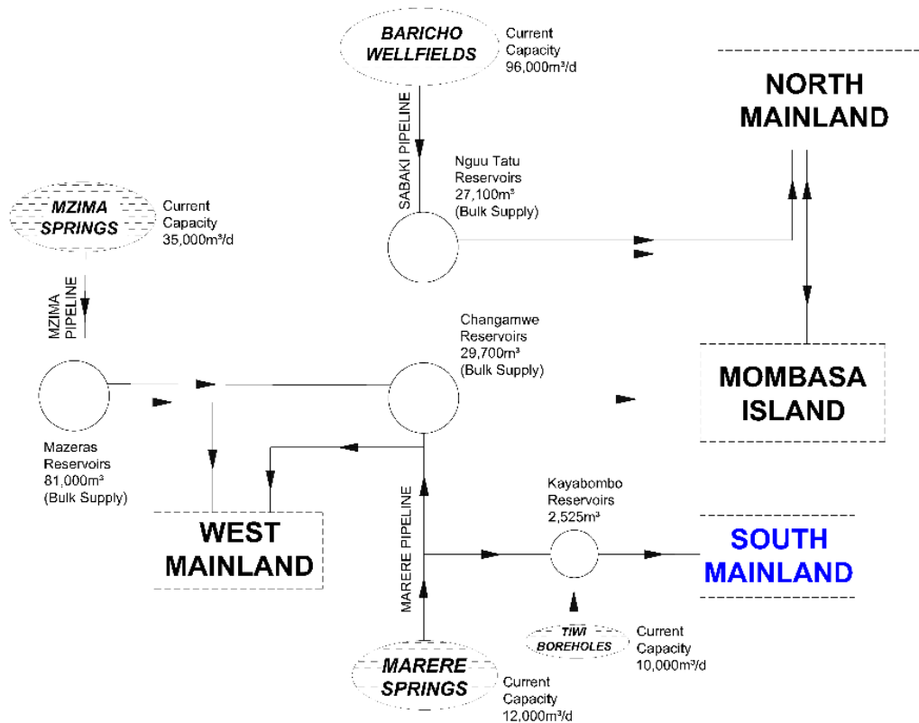
Figure 2.2: Schematic Layout of the Existing Water Supply System for Mombasa County
