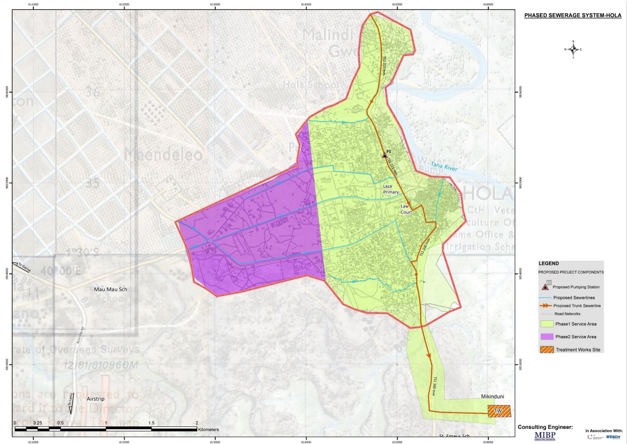
Figure 7.2: Proposed Wastewater Management Scheme for HOLA TOWN
