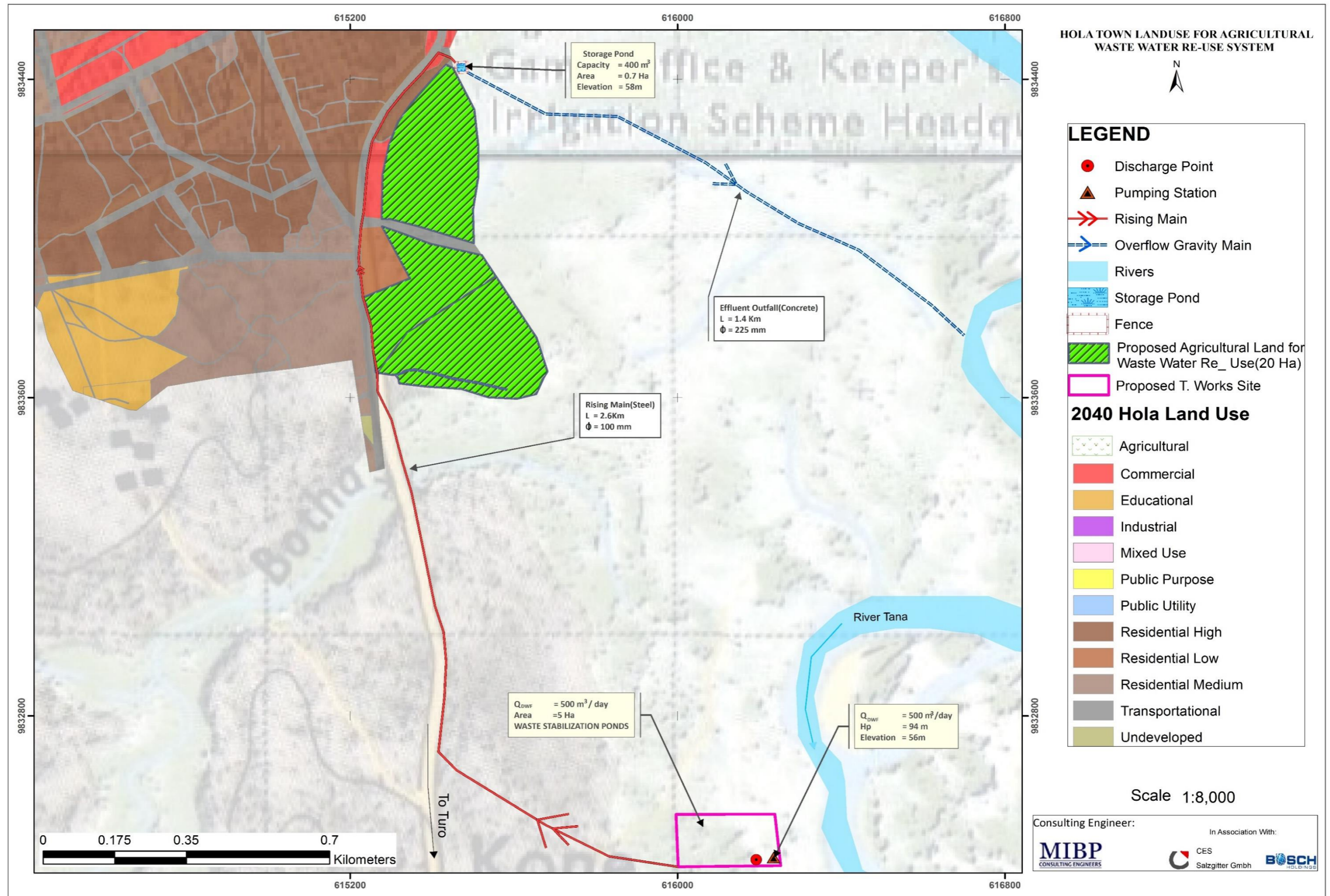
Figure 10.8: Layout Plan of the Conveyance and Storage System for Agricultural Wastewater Reuse – Hola Town
